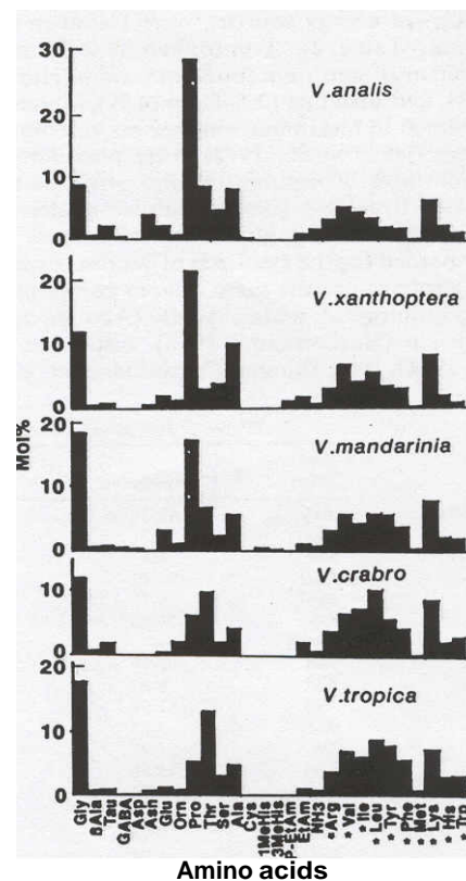
Fig. 1. Molar ratio of amino acids contained in hornet larval saliva. Twenty-eight amino acids as shown in the figure were determined in the larval saliva of five species *• Is essential amino acids.
